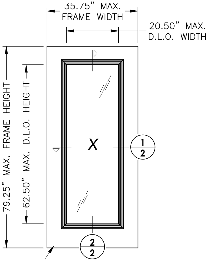
LIGHT DETAIL
